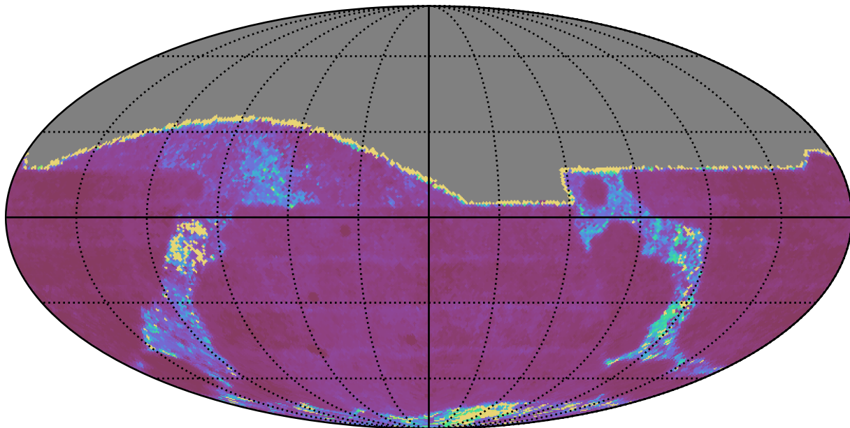
weather_cloudso30v3.4_10yrs All sky g band: Median Inter-Night Gap
