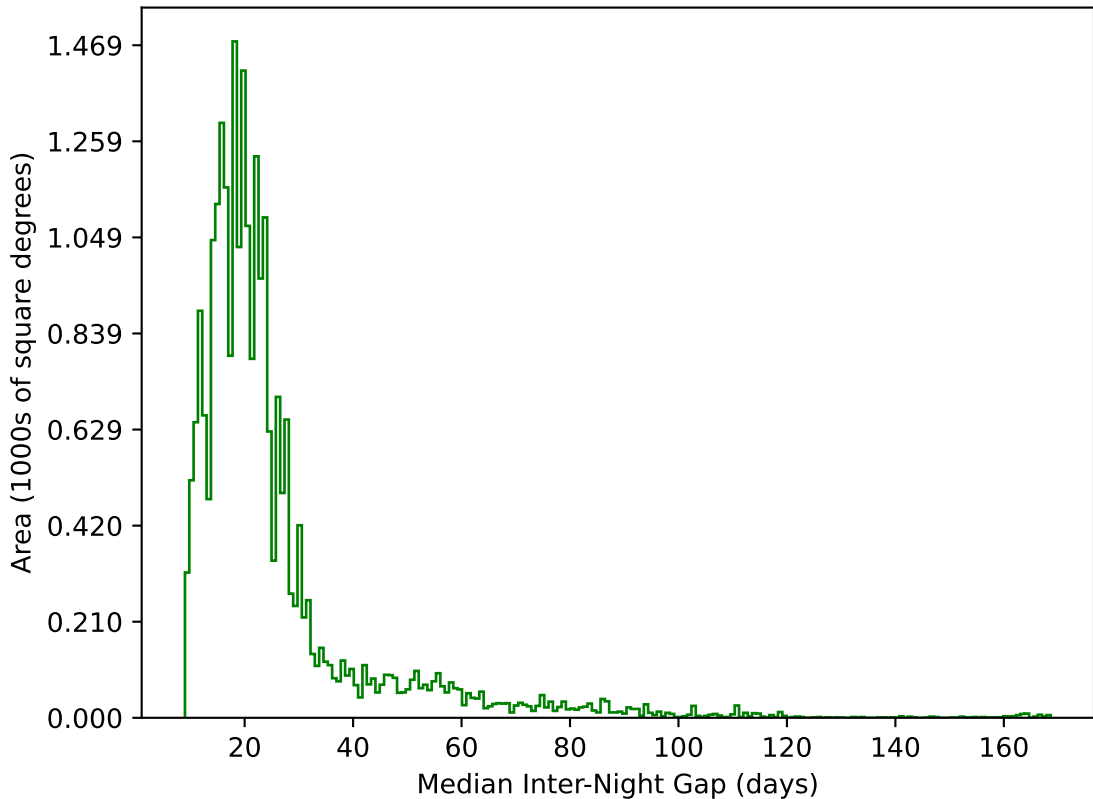
weather_cloudso30v3.4_10yrs All sky g band: Median Inter-Night Gap
