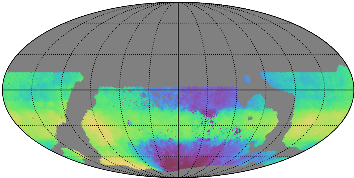
weather_cloudso30v3.4_10yrs WFD z band: Median HA
