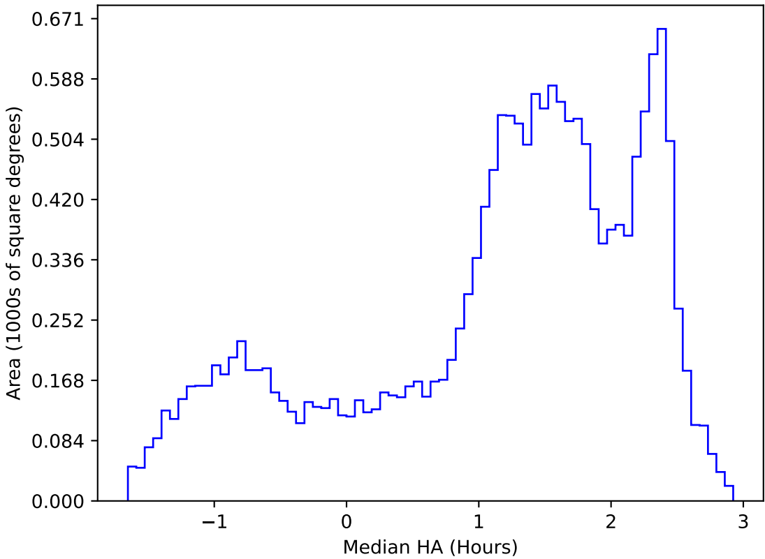
weather_cloudso30v3.4_10yrs WFD y band: Median HA
