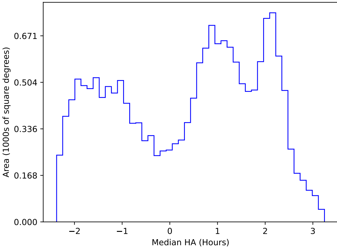
weather_cloudso30v3.4_10yrs WFD u band: Median HA
