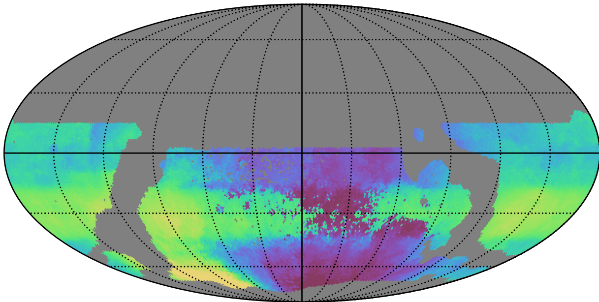
weather_cloudso30v3.4_10yrs WFD r band: Median HA
