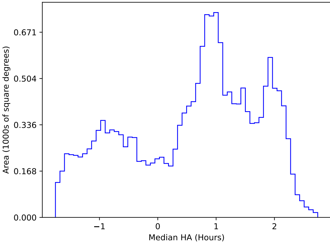
weather_cloudso30v3.4_10yrs WFD r band: Median HA
