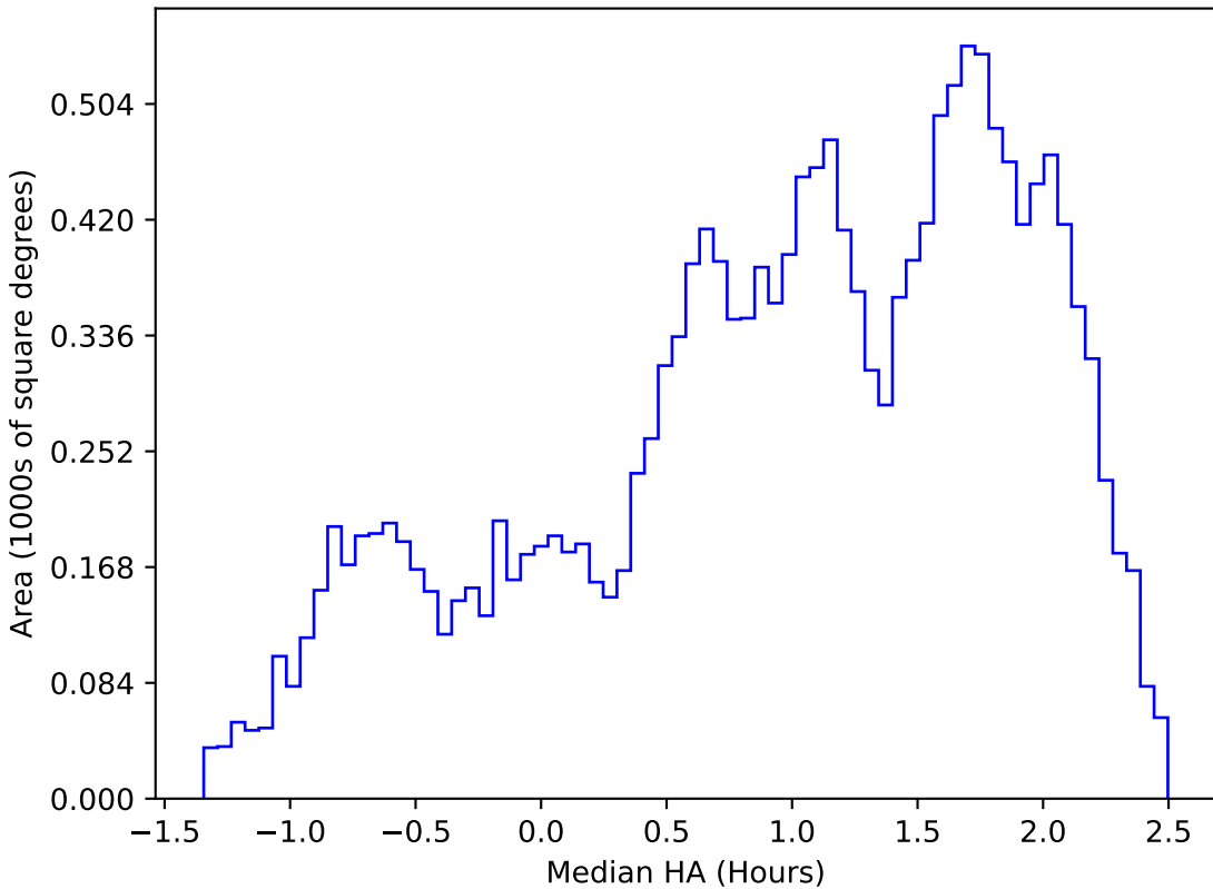
weather_cloudso30v3.4_10yrs WFD i band: Median HA
