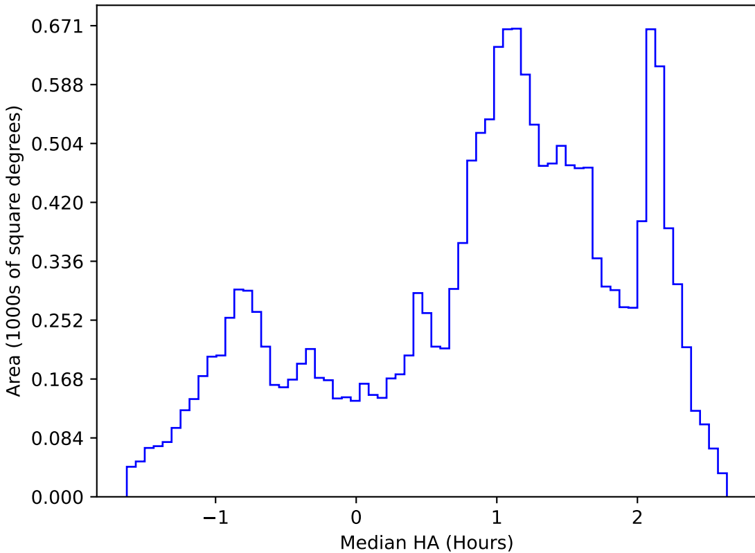
weather_cloudso30v3.4_10yrs WFD all bands: Median HA
