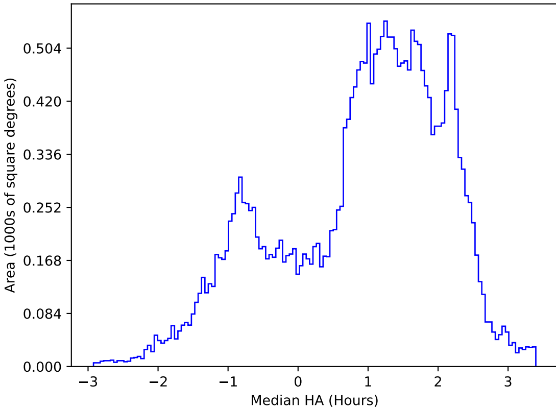
weather_cloudso30v3.4_10yrs All sky z band: Median HA
