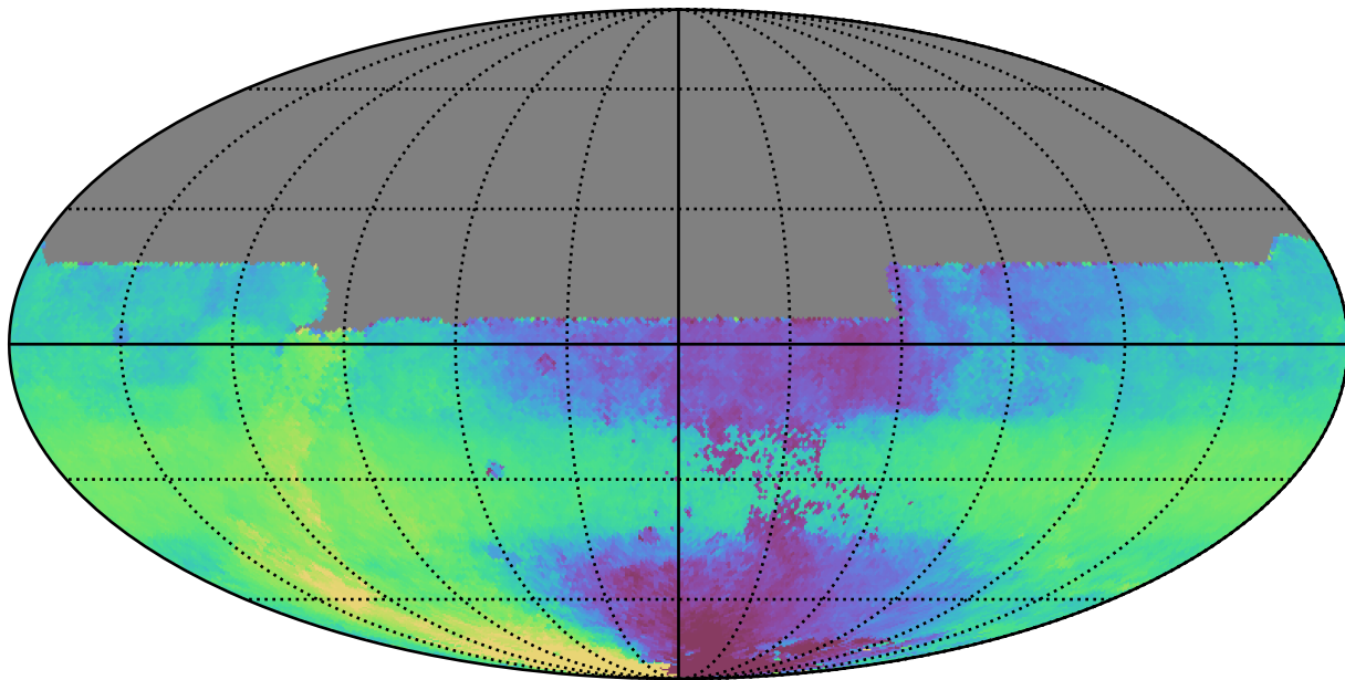
weather_cloudso30v3.4_10yrs All sky y band: Median HA
