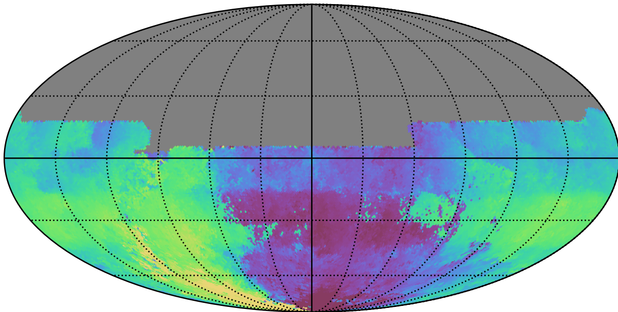
weather_cloudso30v3.4_10yrs All sky u band: Median HA
