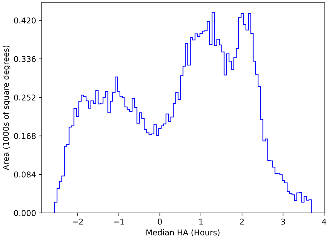
weather_cloudso30v3.4_10yrs All sky u band: Median HA
