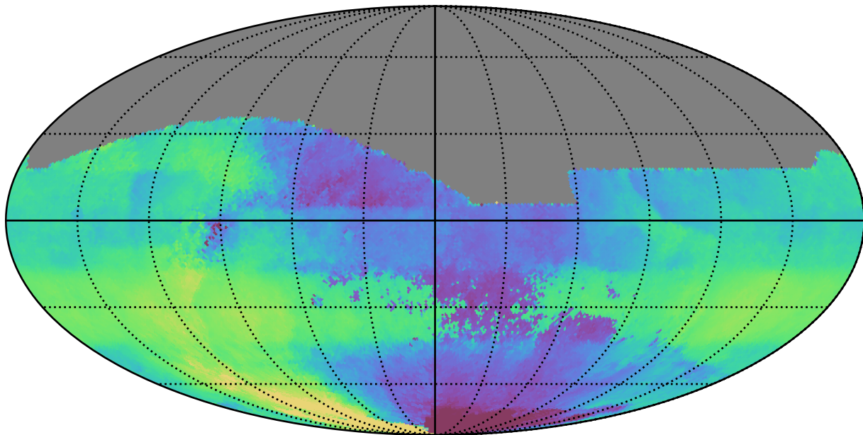
weather_cloudso30v3.4_10yrs All sky r band: Median HA
