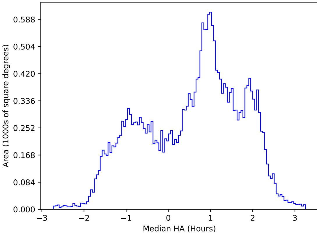
weather_cloudso30v3.4_10yrs All sky r band: Median HA
