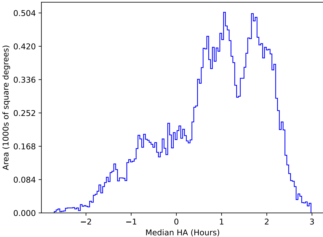
weather_cloudso30v3.4_10yrs All sky i band: Median HA
