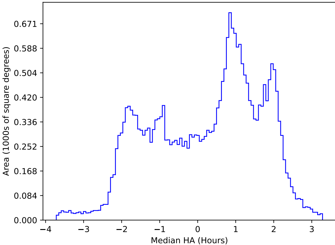
weather_cloudso30v3.4_10yrs All sky g band: Median HA
