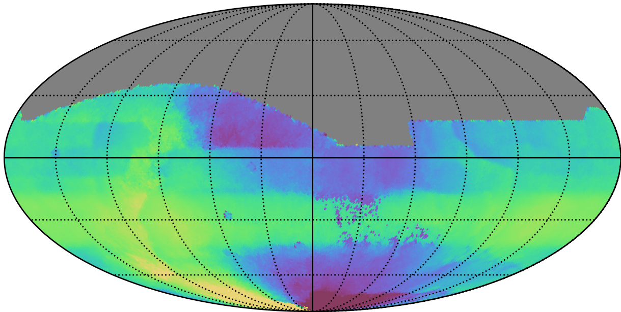
weather_cloudso30v3.4_10yrs All sky all bands: Median HA
