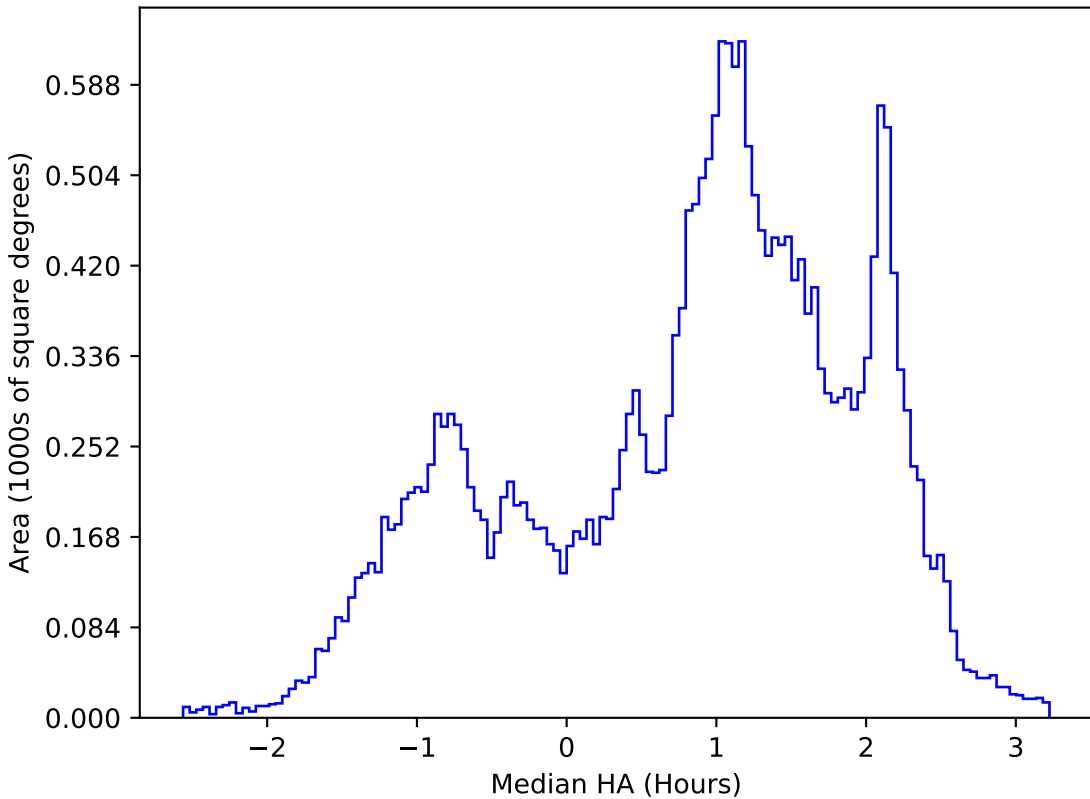
weather_cloudso30v3.4_10yrs All sky all bands: Median HA
