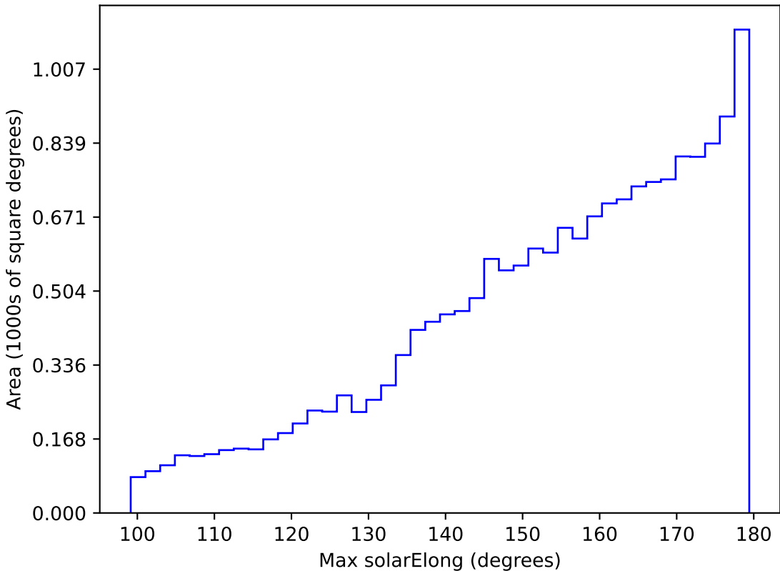
weather_cloudso30v3.4_10yrs WFD z band: Max solarElong
