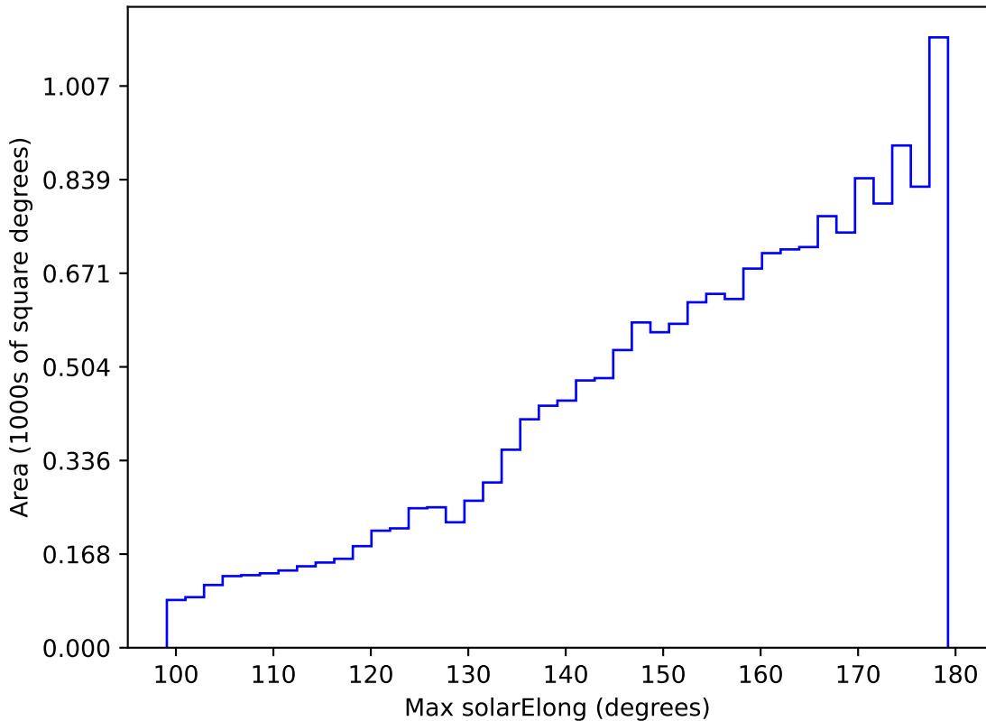
weather_cloudso30v3.4_10yrs WFD y band: Max solarElong
