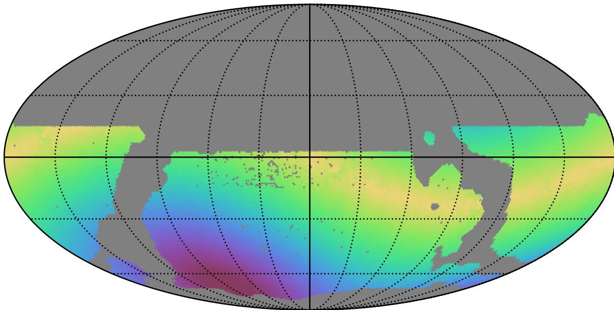
weather_cloudso30v3.4_10yrs WFD u band: Max solarElong
