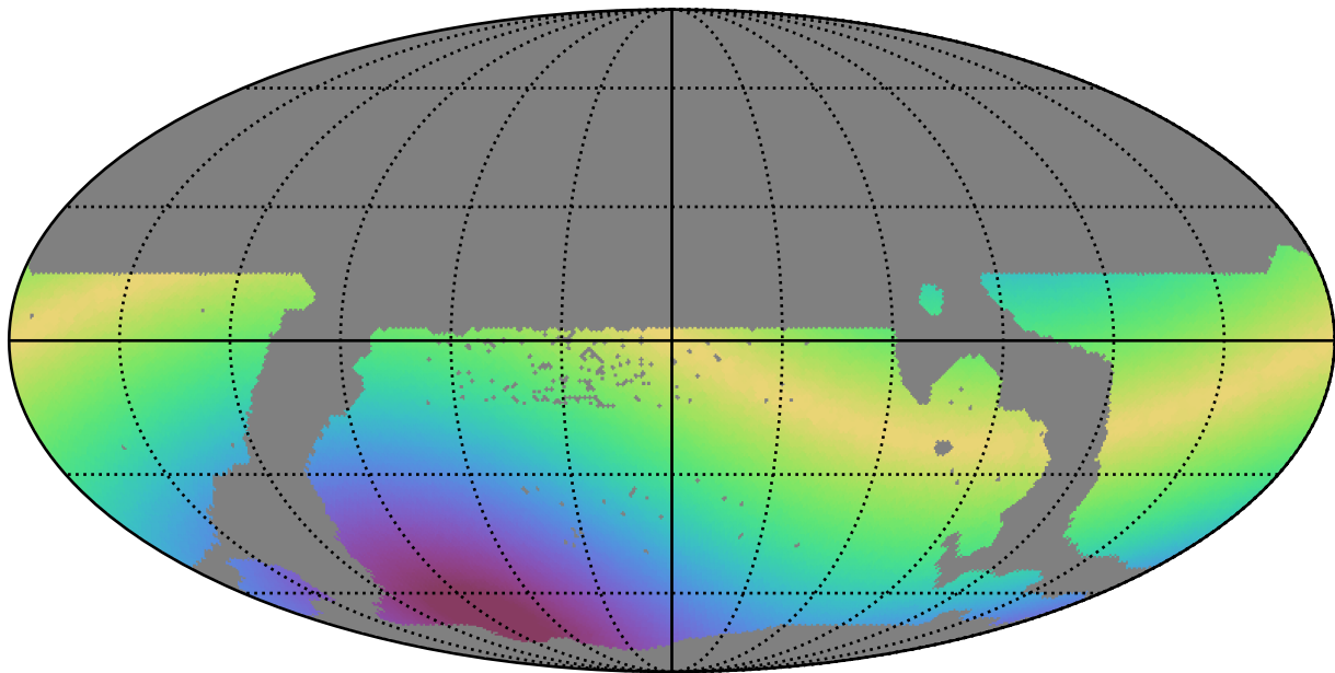
weather_cloudso30v3.4_10yrs WFD r band: Max solarElong
