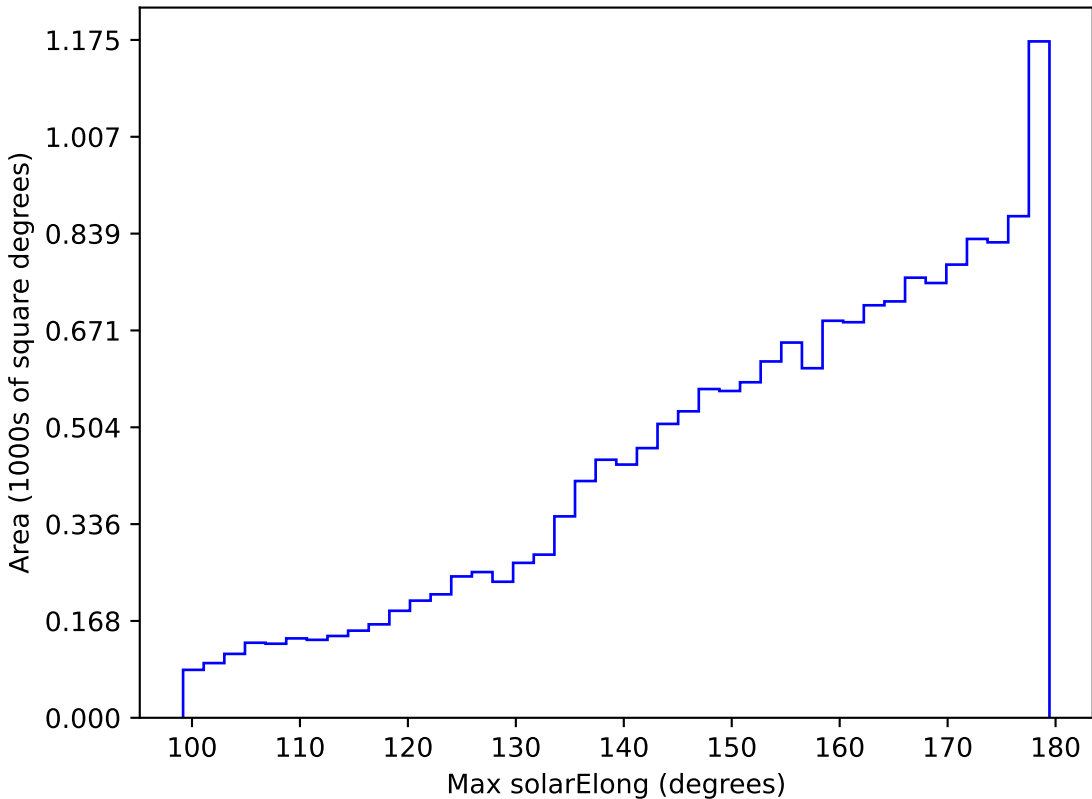
weather_cloudso30v3.4_10yrs WFD r band: Max solarElong
