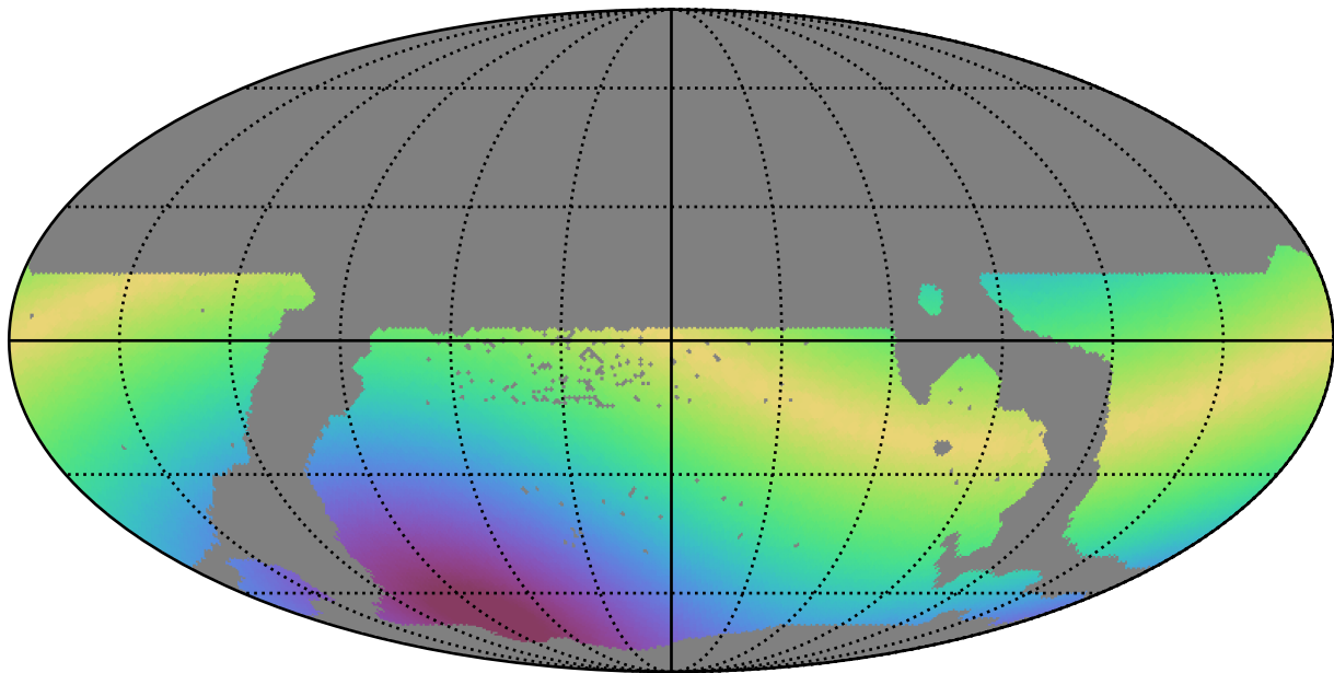
weather_cloudso30v3.4_10yrs WFD i band: Max solarElong
