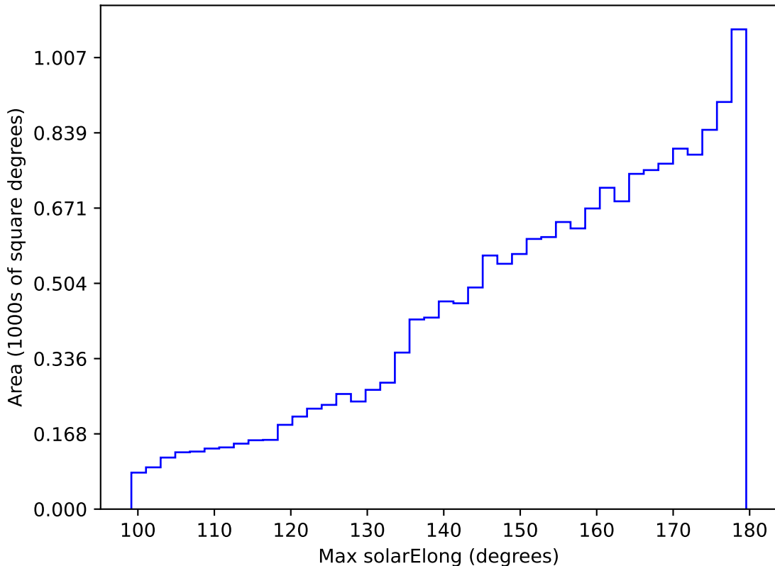
weather_cloudso30v3.4_10yrs WFD i band: Max solarElong
