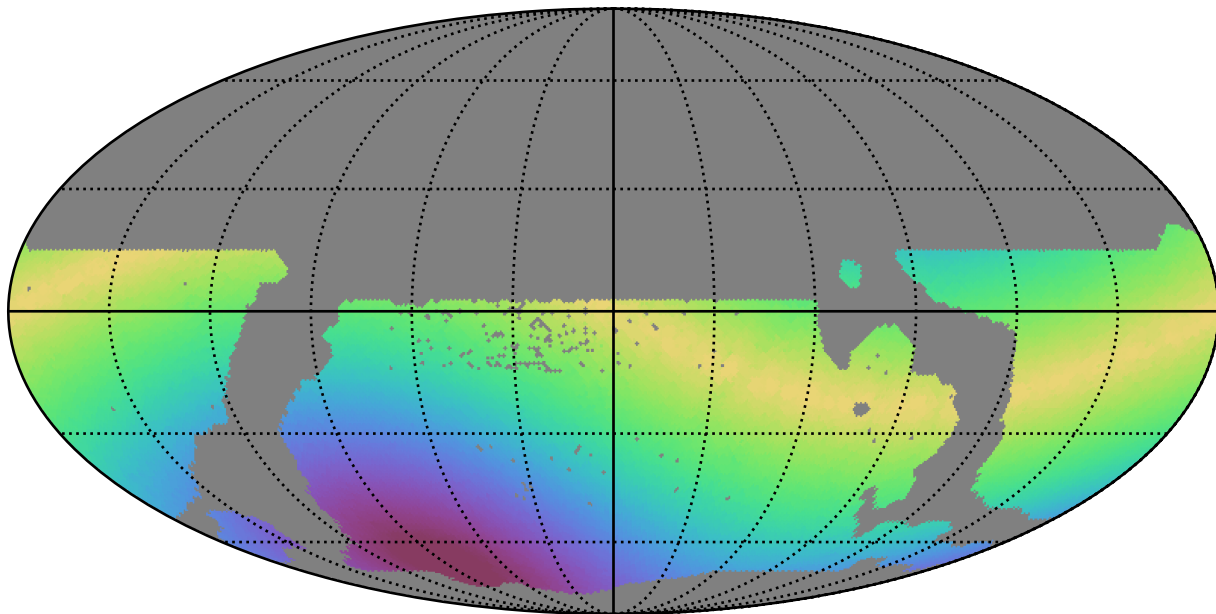
weather_cloudso30v3.4_10yrs WFD g band: Max solarElong
