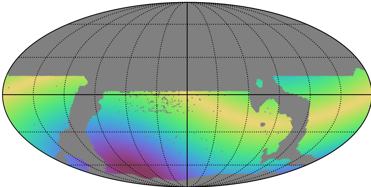
weather_cloudso30v3.4_10yrs WFD all bands: Max solarElong
