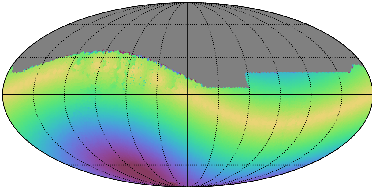
weather_cloudso30v3.4_10yrs All sky z band: Max solarElong
