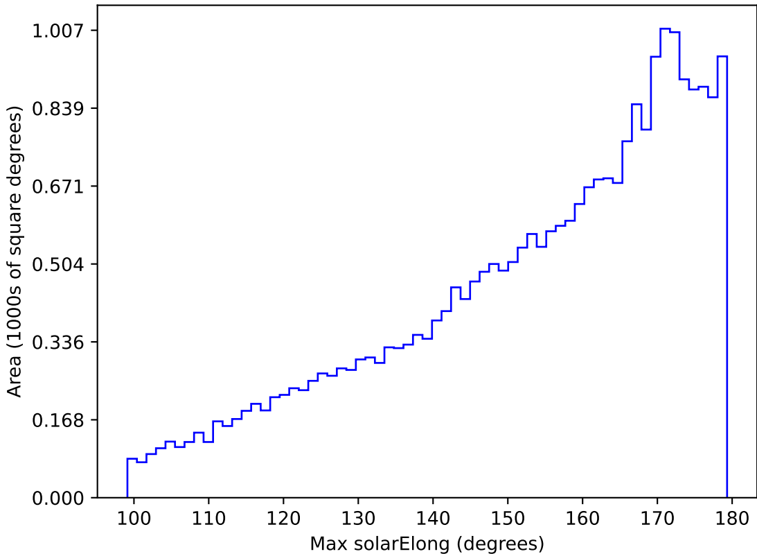
weather_cloudso30v3.4_10yrs All sky z band: Max solarElong
