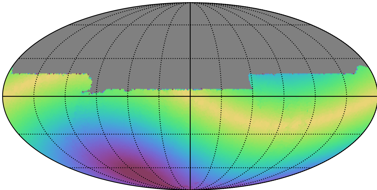
weather_cloudso30v3.4_10yrs All sky y band: Max solarElong
