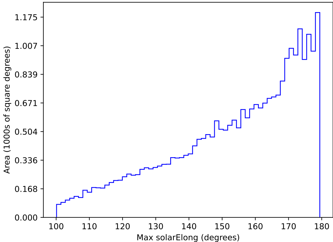
weather_cloudso30v3.4_10yrs All sky r band: Max solarElong
