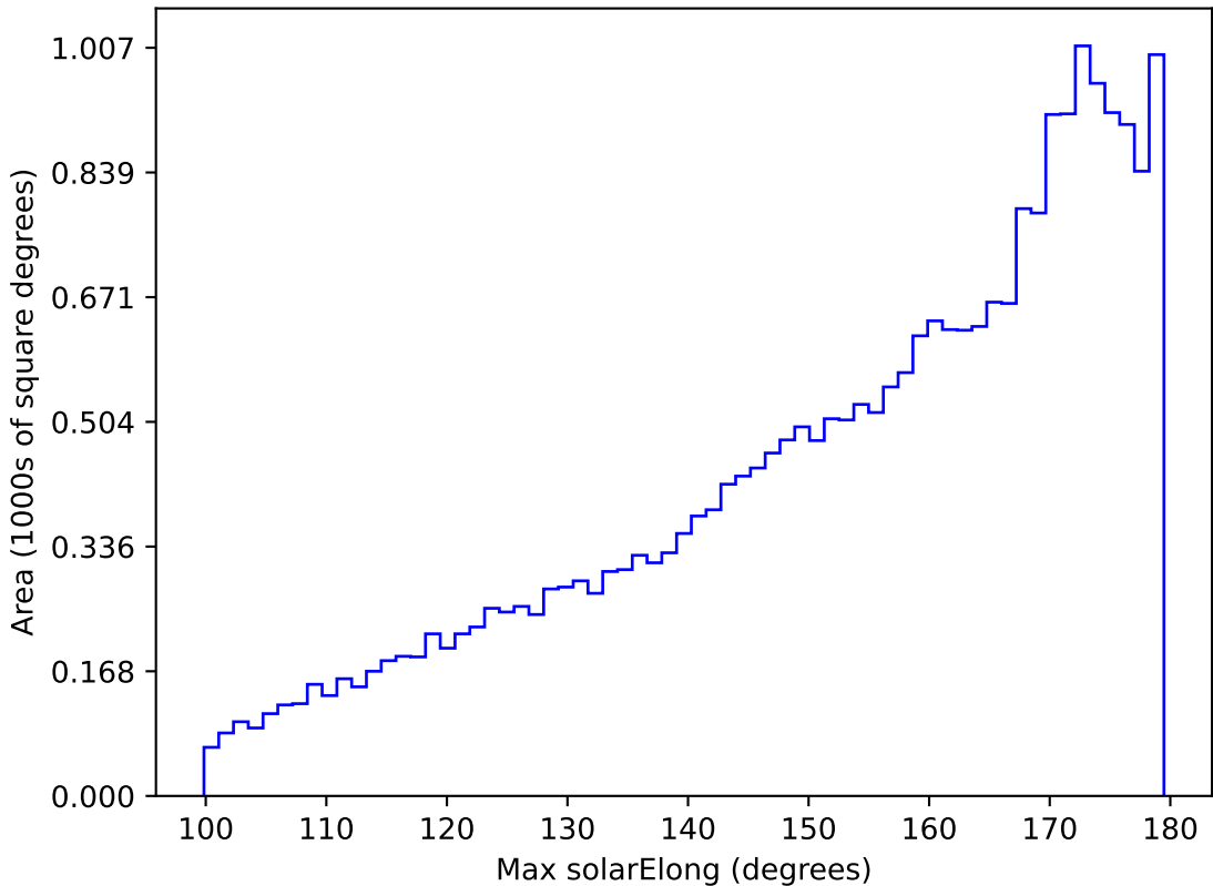
weather_cloudso30v3.4_10yrs All sky i band: Max solarElong
