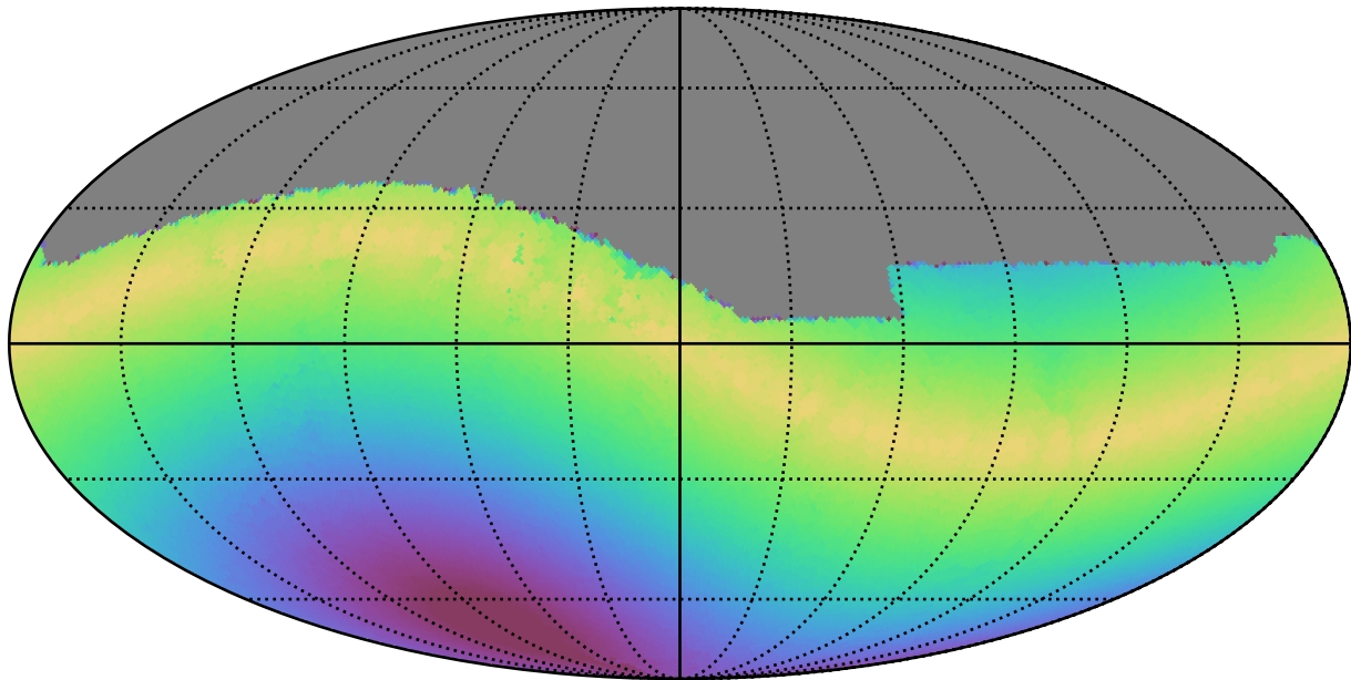
weather_cloudso30v3.4_10yrs All sky g band: Max solarElong
