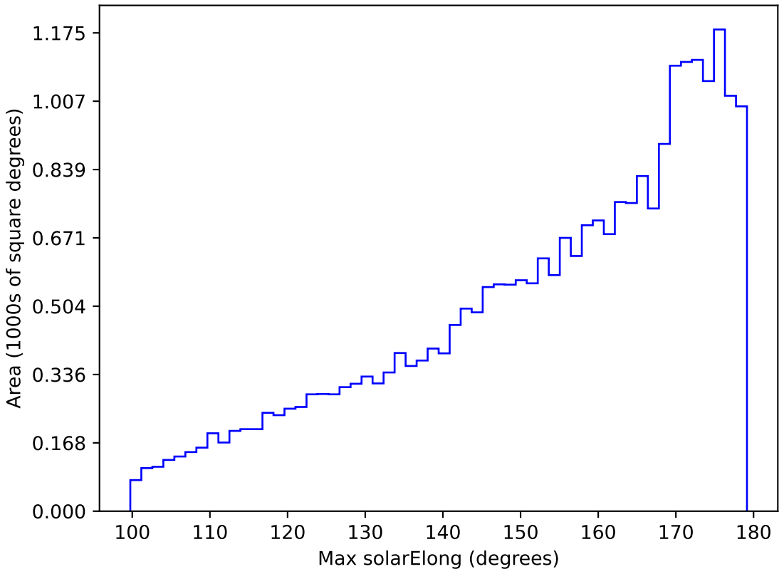
weather_cloudso30v3.4_10yrs All sky g band: Max solarElong
