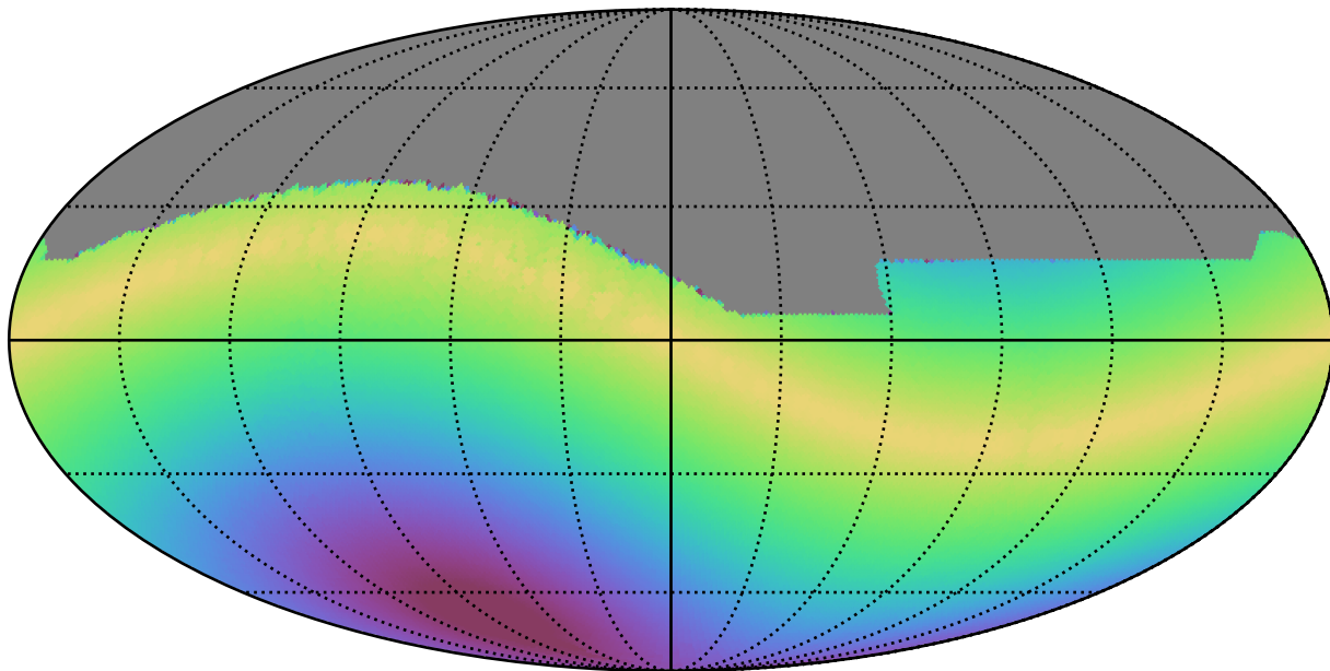
weather_cloudso30v3.4_10yrs All sky all bands: Max solarElong
