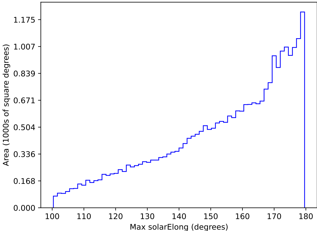
weather_cloudso30v3.4_10yrs All sky all bands: Max solarElong
