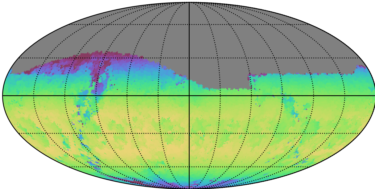
weather_cloudso30v3.4_10yrs Yr 1 z band: Max skyBrightness
