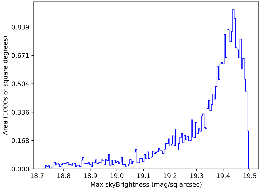
weather_cloudso30v3.4_10yrs Yr 1 z band: Max skyBrightness
