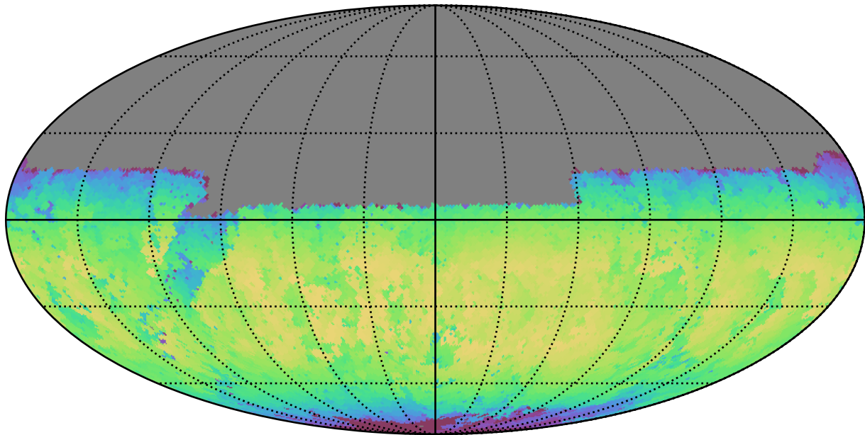
weather_cloudso30v3.4_10yrs Yr 1 y band: Max skyBrightness
