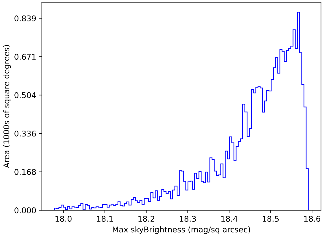
weather_cloudso30v3.4_10yrs Yr 1 y band: Max skyBrightness
