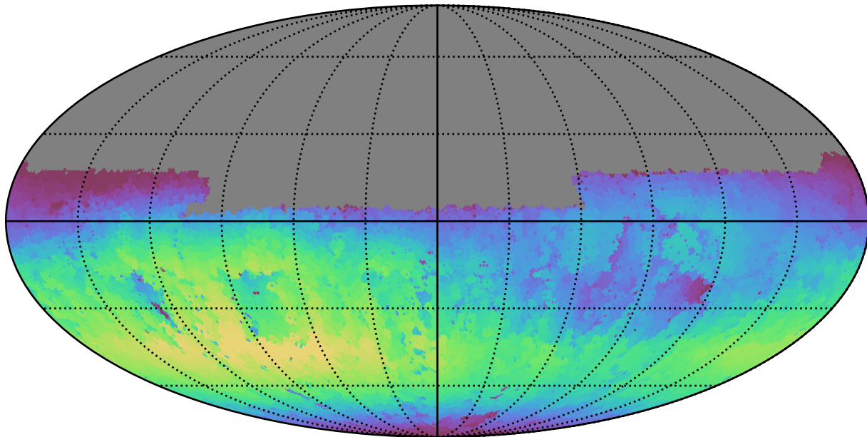
weather_cloudso30v3.4_10yrs Yr 1 u band: Max skyBrightness
