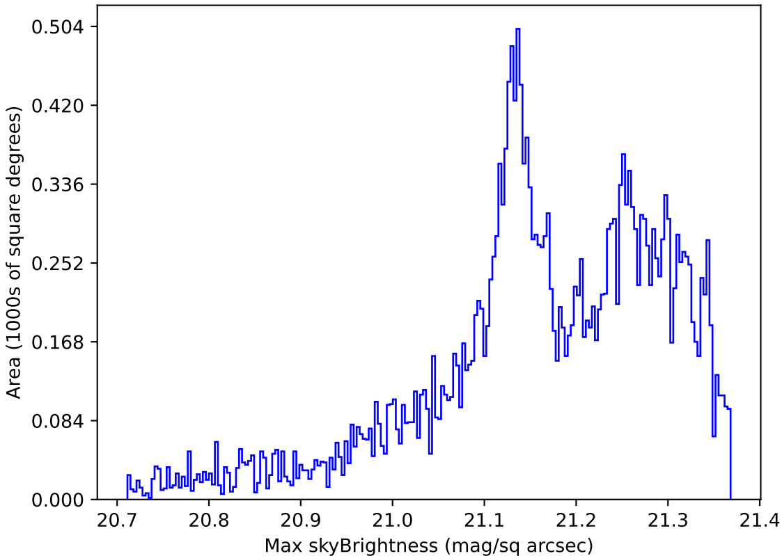
weather_cloudso30v3.4_10yrs Yr 1 r band: Max skyBrightness
