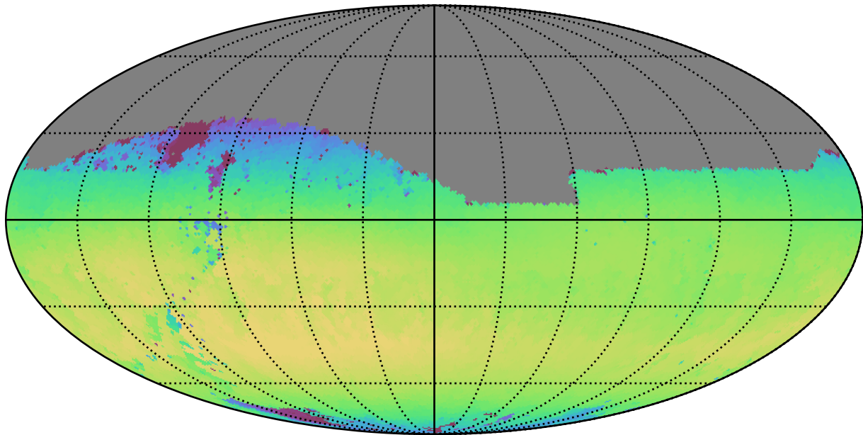
weather_cloudso30v3.4_10yrs Yr 1 i band: Max skyBrightness
