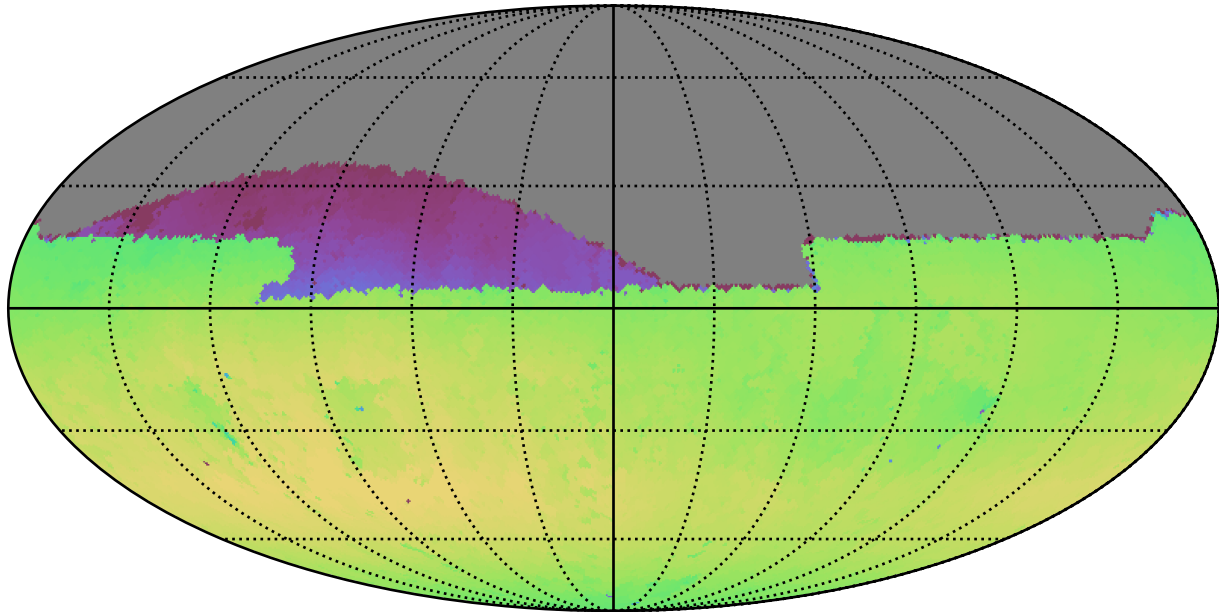
weather_cloudso30v3.4_10yrs Yr 1 all bands: Max skyBrightness
