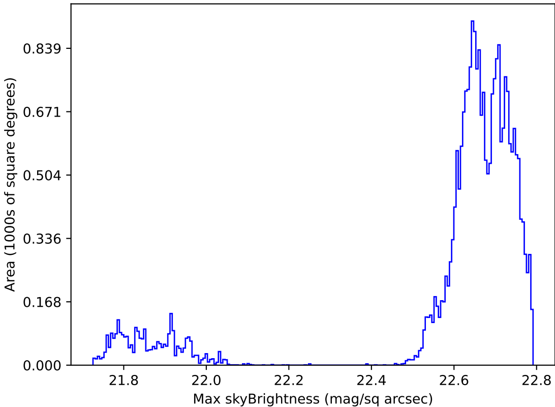
weather_cloudso30v3.4_10yrs Yr 1 all bands: Max skyBrightness
