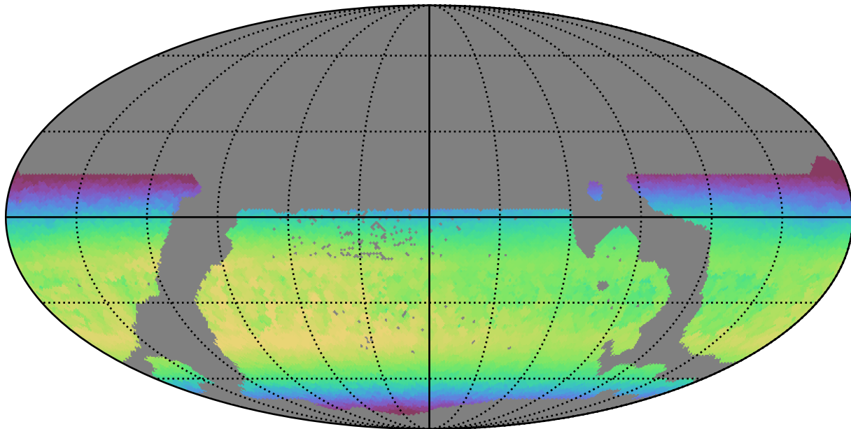
weather_cloudso30v3.4_10yrs WFD z band: Max skyBrightness
