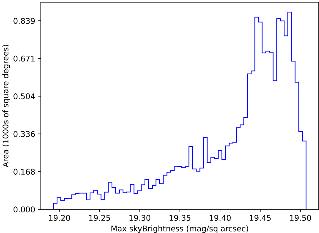
weather_cloudso30v3.4_10yrs WFD z band: Max skyBrightness
