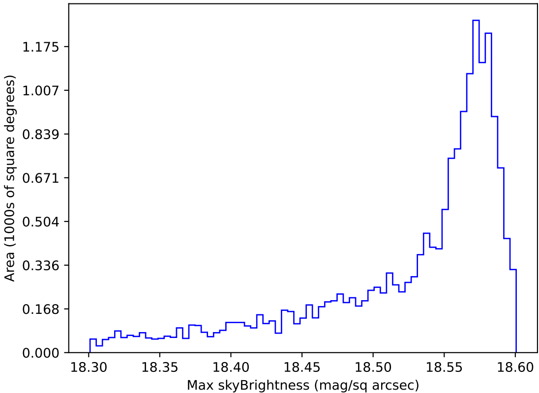
weather_cloudso30v3.4_10yrs WFD y band: Max skyBrightness
