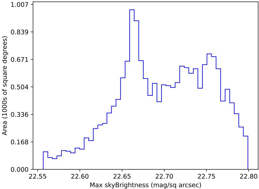
weather_cloudso30v3.4_10yrs WFD u band: Max skyBrightness
